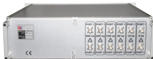
(b) TLP-8012A5 back side
