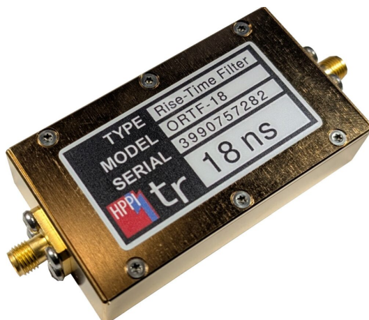
Figure 3: ORTF-18 (size: 67.2 mm x 37.2 mm x 16.8 mm)
