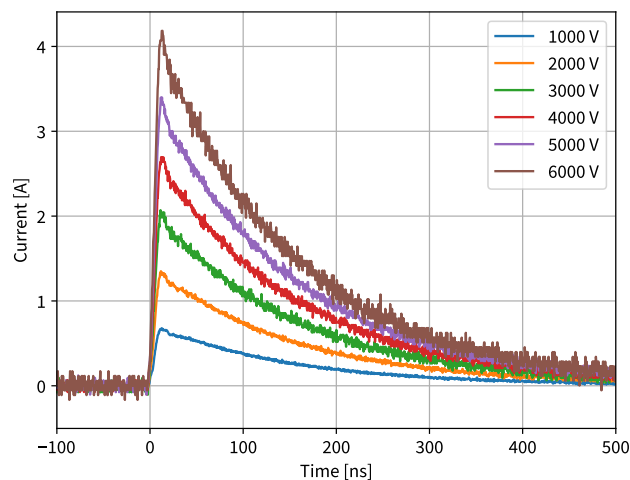
(b) Measured 1 kV to 6 kV HBM level sweep into short circuit
