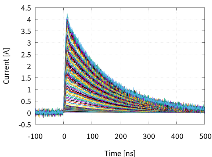
(a) Measured 30 V to 6 kV HBM level sweep into short circuit
