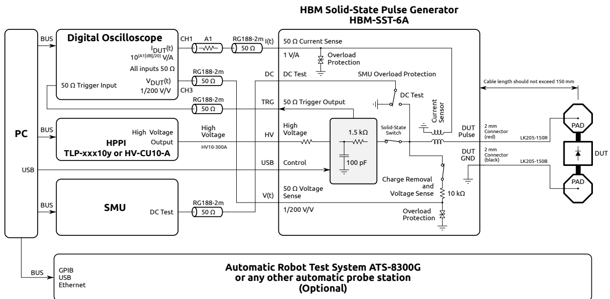
Figure 1: Typical 2-wire HBM measurement setup using the HBM-SST-6A pulse generator
