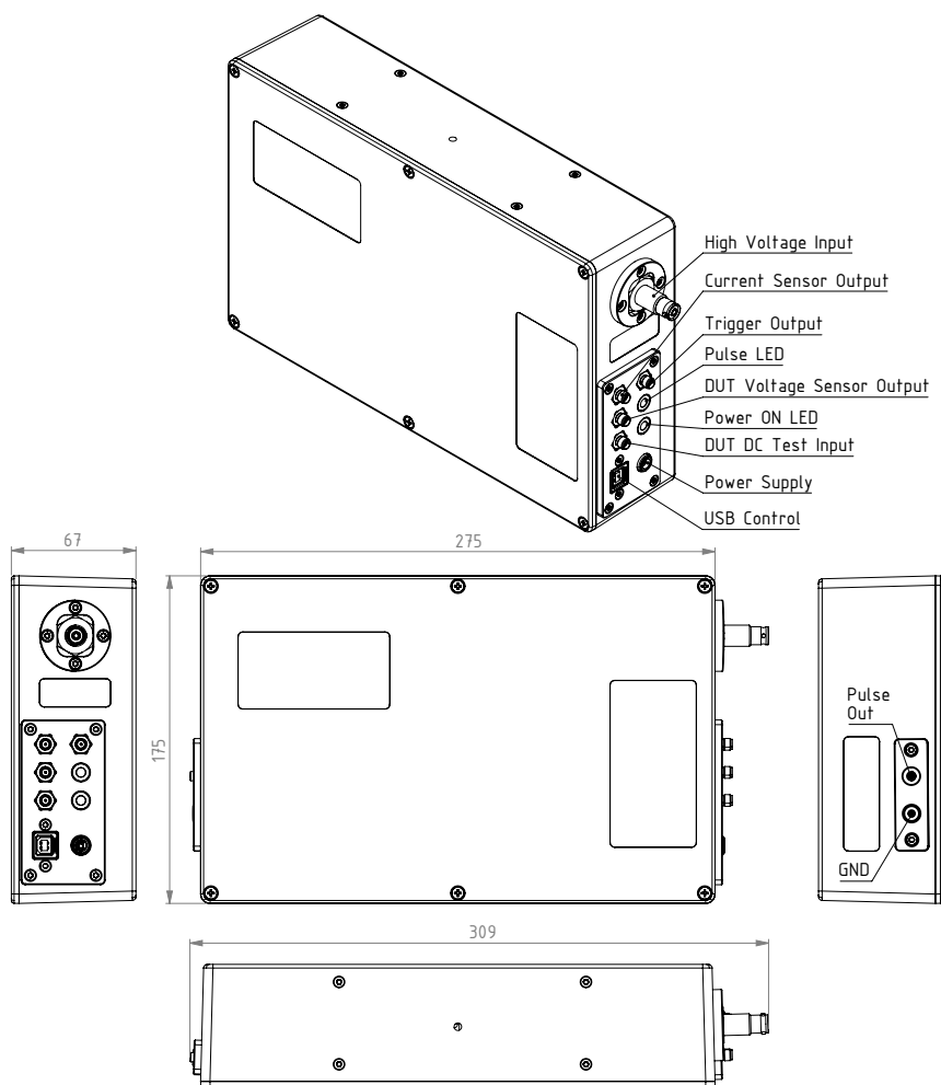
Figure 5: HBM-SST-6A physical dimensions in [mm].
