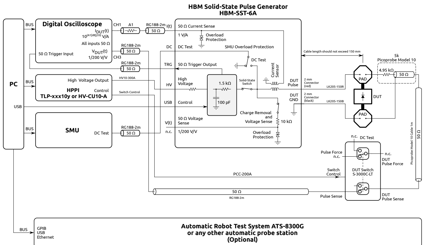
Figure 2: Typical 4-wire (Kelvin) HBM measurement setup using the HBM-SST-6A pulse generator
